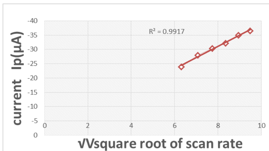
Figure (7): Graph of current versus square root of scan rate in the acid medium HCl.
