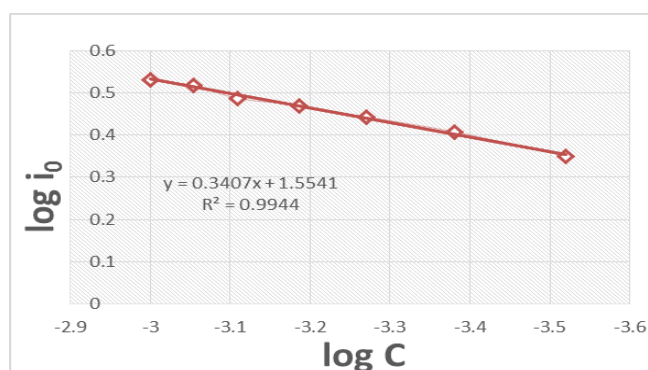
Figure(4): Graph of \log(i_0) of \log(C) in HCl.
