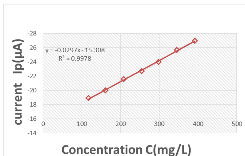
Figure (8): Graph of the limit of the current with different concentrations of Pioglitazone Hydrochloride in the acid medium.
