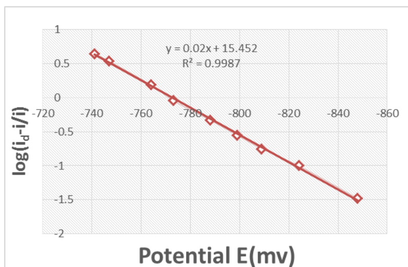
Figure (5): Graph of \log(i_d - i/i) of E(mv) in HCl.
