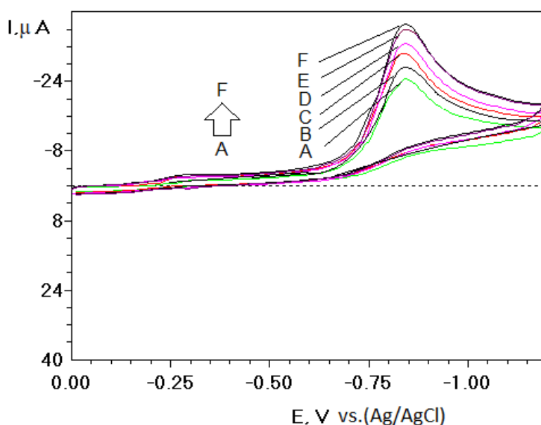
Figure (6): Cyclic voltammograms of Pioglitazone Hydrochloride at different scan rate (40 to 90 mV/s) in HCl.
