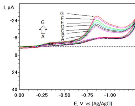
Figure (2): Cyclic voltammetry curves for different concentrations of Pioglitazone Hydrochloride (A: 117 - B: 161 - C: 208 - D: 255 - E: 298 - F: 345 - G: 392 mg/L) in HCl at gold electrode.
