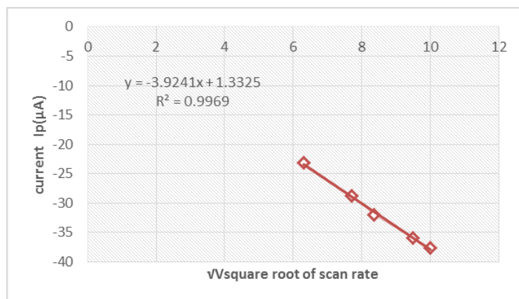
Figure(7) Graph of current versus square root of scan rate in the acid medium HCl(0.5M).
