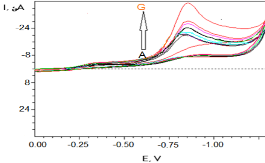
Figure(2) Cyclic voltammetry curves for different concentrations of Pioglitazone Hydrochloride.
