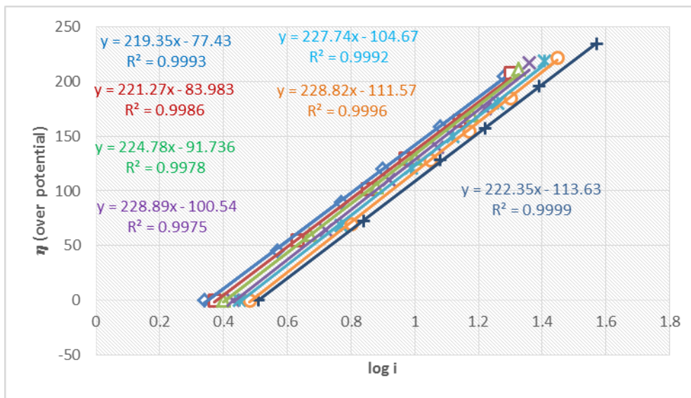
Figure(3) Graph of \eta of \log(i) for different concentrations of Pioglitazone Hydrochloride.
