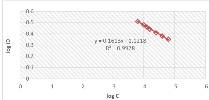
Figure(4) Graph of \log(i_0) of \log(C) in HCl (0.5M).
