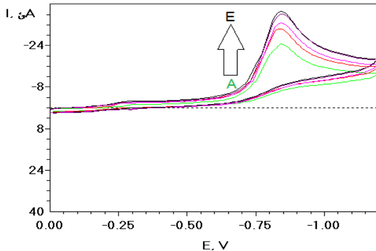
Figure (6) Cyclic voltammograms of Pioglitazone Hydrochloride at different scan rate (40 to 100 mV/s) in HCl(0.5M).
