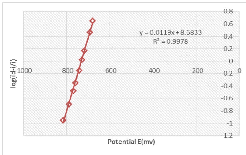
Figure(5) Graph of \log(i_d - i/i) of E(mv) in HCl(0.5M)
