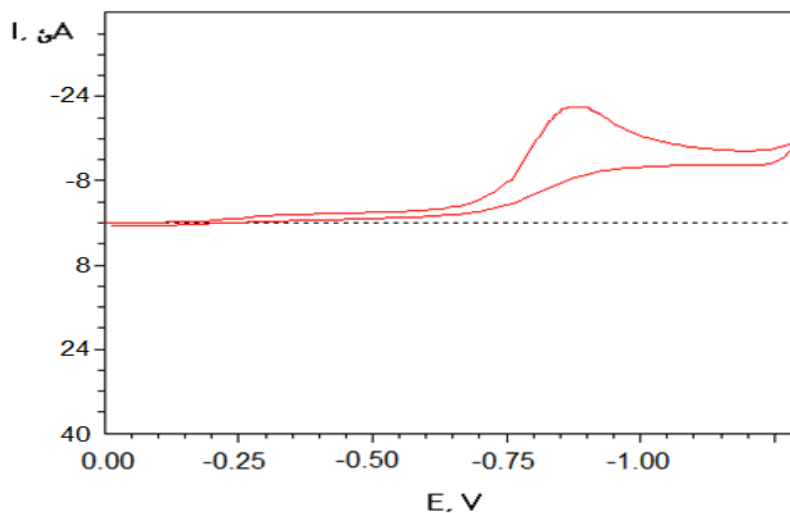
Figure(9) cyclic voltammetry of the electrochemical reduction of a Defast sample in the acid medium HCl(0.5 M) on a gold electrode with a scan rate (50mv/s)
